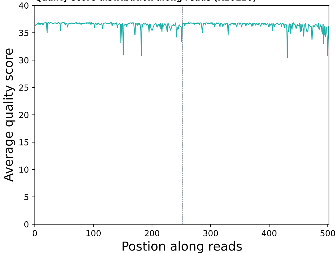
Quality score distribution along reads (R20120)
